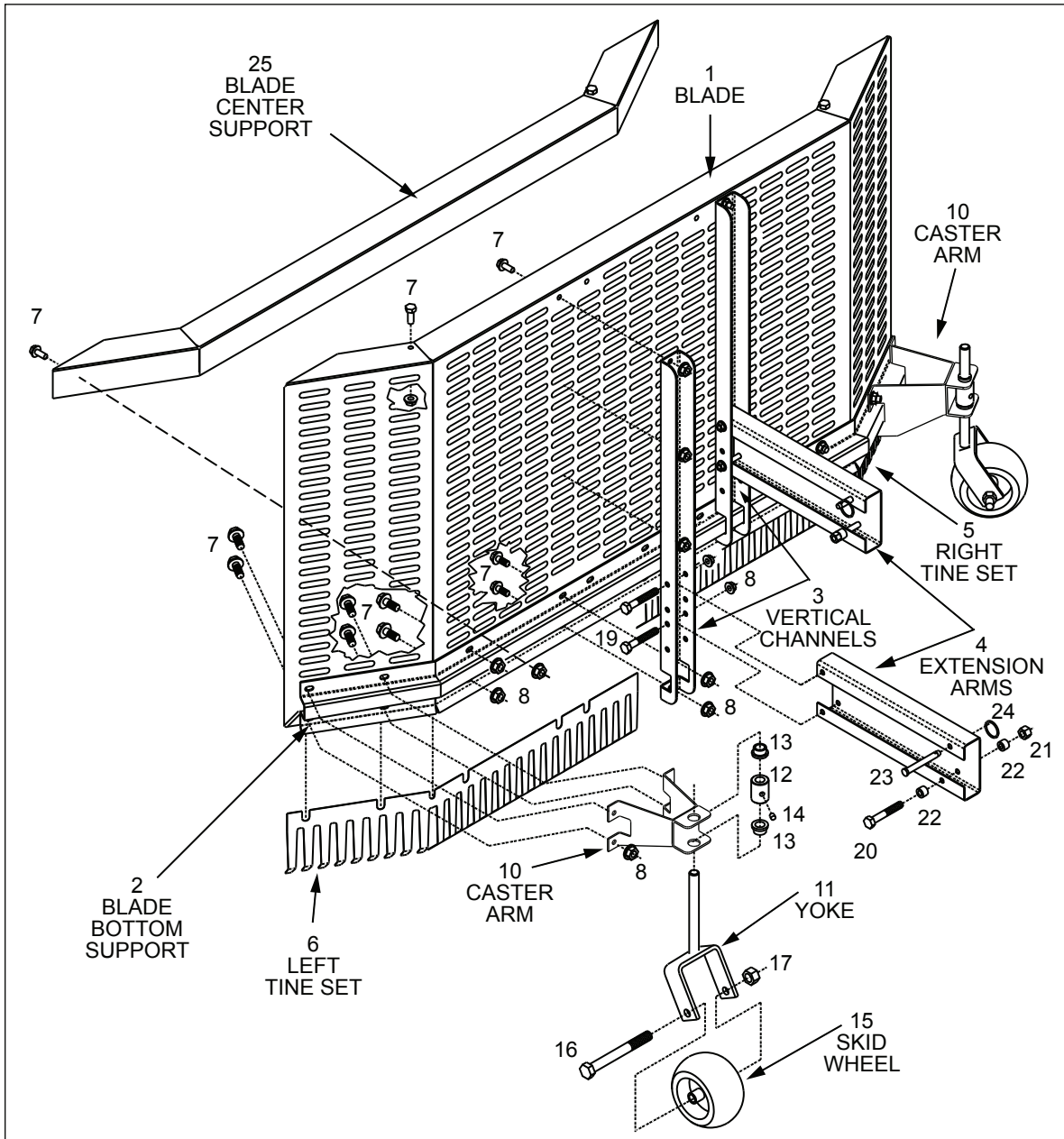
Fig. 1. JRCO LEAF BLADE Plow Parts Drawing
